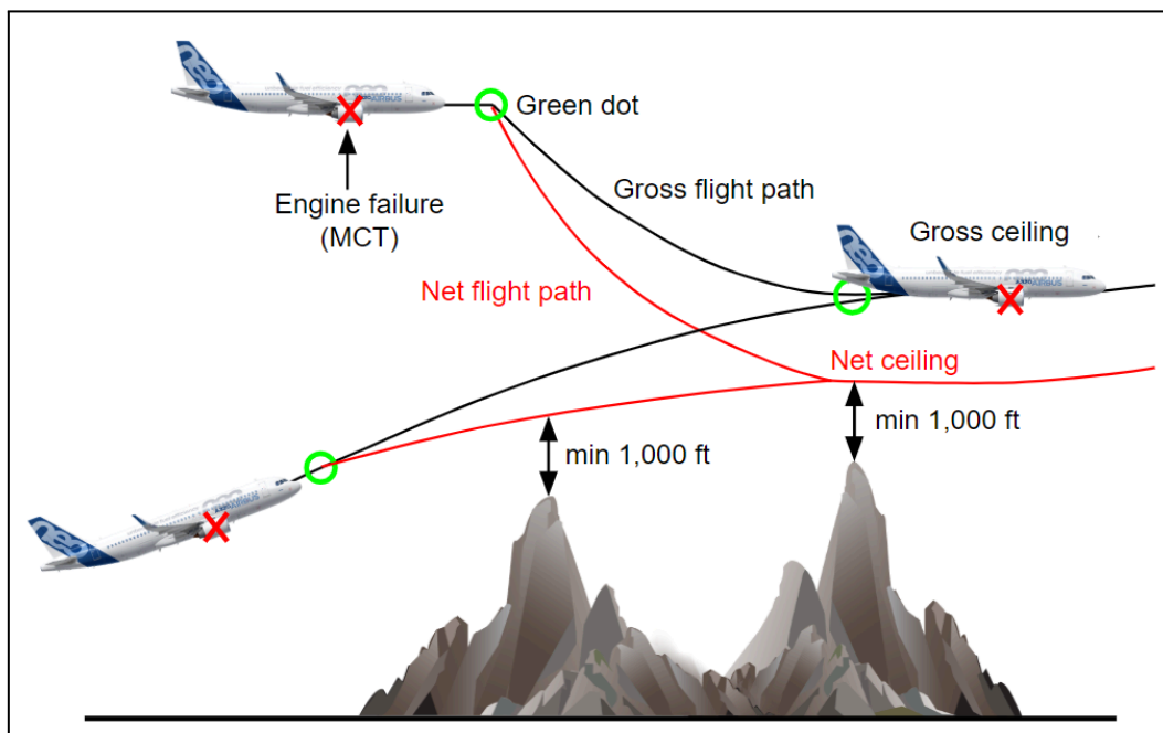
Illustration E-4: Vertical Clearance (1,000 feet)
