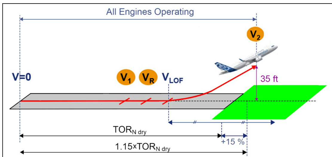
Illustration C-16: TOR N dry
