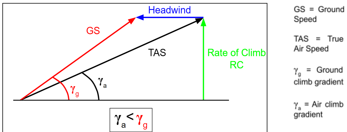
Illustration D-4: Headwind Component in Climb
