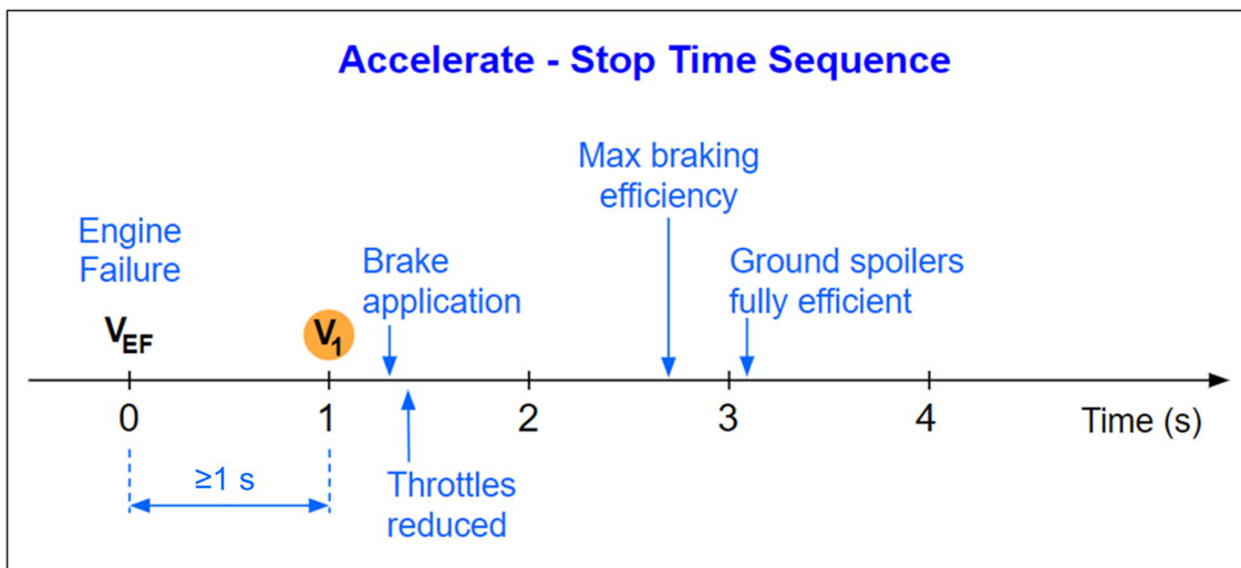
Illustration C-19: Example of Accelerate - Stop Time Sequence
