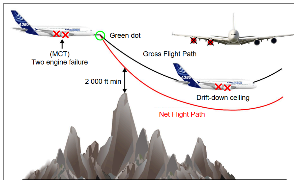
Illustration E-7: Obstacle Clearance 2 000 feet – Two Engines Inoperative
