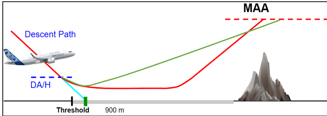
Illustration F-22: Effect of Go-Around Speed Optimization (in red with speed optimization, in green without speed optimization)
