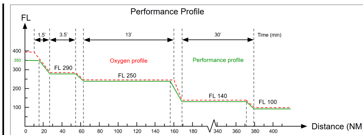
Illustration E-11: A319 Performance Profile – Oxygen System that Lasts for 22 Minutes - Air OPS CAT.IDE.A.230 allowance
