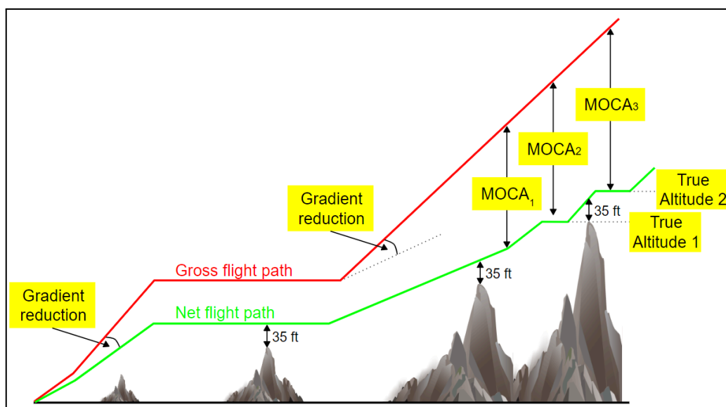
Illustration C-26: Method 4 for Obstacles Clearance
