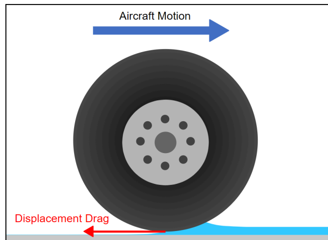
Illustration C-52: Displacement Drag
