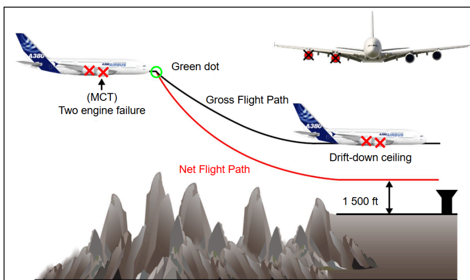
Illustration E-8: Performance Requirement above Diversion Airport
