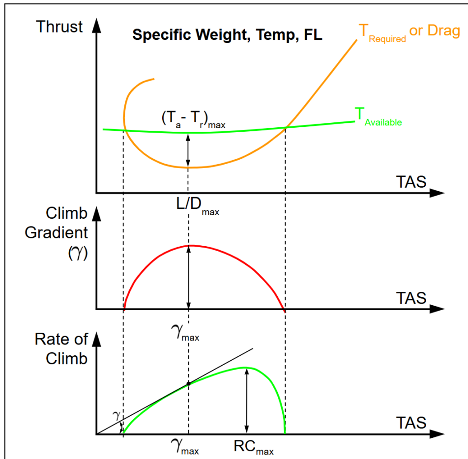
Illustration A5-6: Thrust Curves and Speed Polar for Climb
