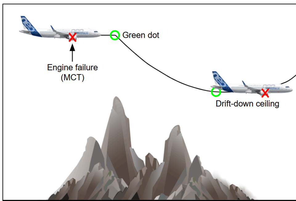
Illustration E-9: Drift-Down Procedure
