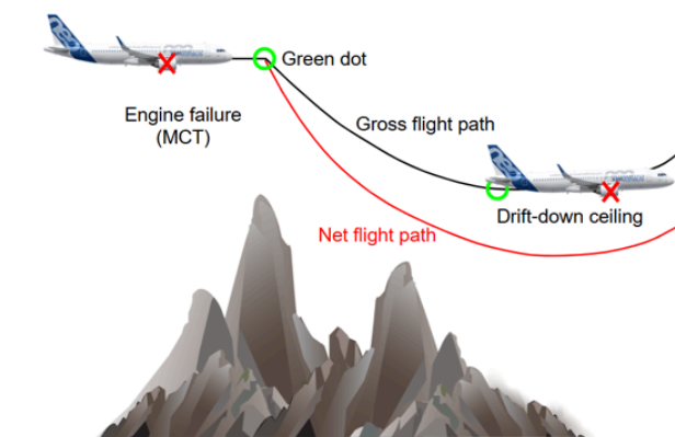
Illustration E-2: Gross and Net Drift-Down Flight Paths (Climb and Descent)
