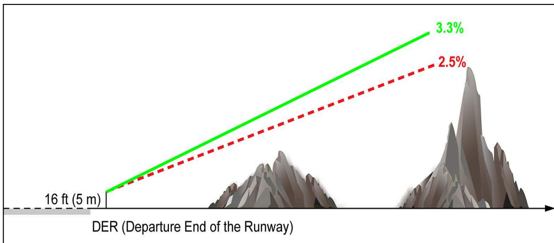
Illustration C-28: AEO Protection Surface
