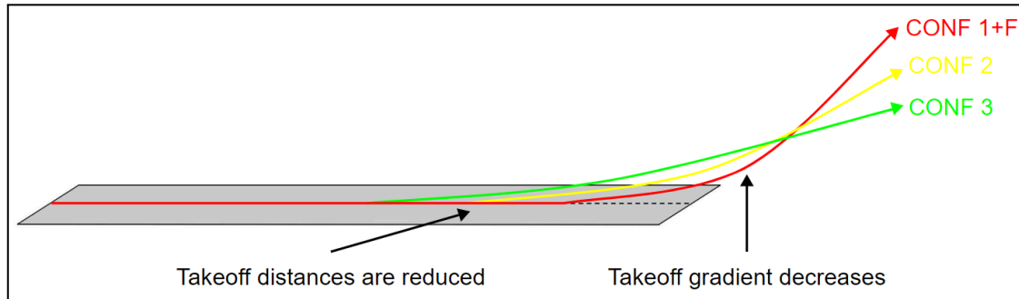
Illustration C-37: Effect of the Flap in the Takeoff Distance and in the Gradient
