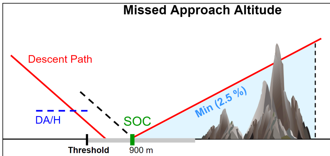
Illustration F-14: Minimum Climb Gradient for Approach not Satisfied due to Obstacle
