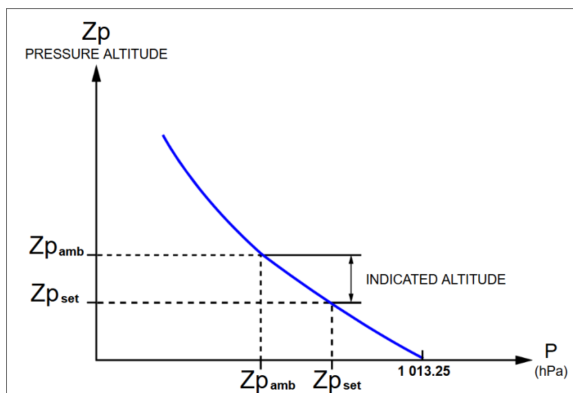
Illustration A3-3: Indicated Altitude (IA)
