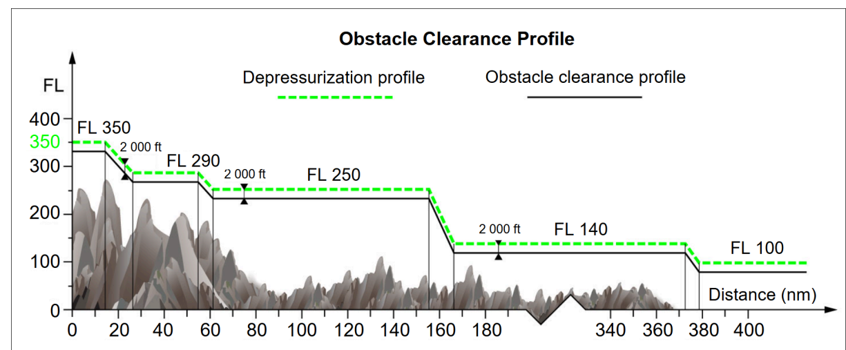
Illustration E-16: A319 Obstacle Clearance Profile - Air OPS CAT.IDE.A.230 allowance included
