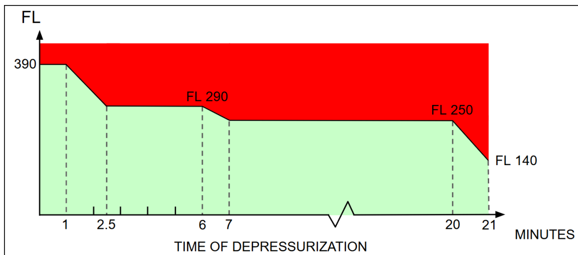
Illustration E-10: A319 Descent Profile - 22 Minute Oxygen System
