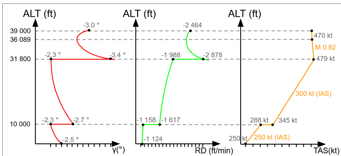
Illustration D-31: A330 Example - Descent Gradient ( \gamma ) and RD Variation with Altitude and TAS
