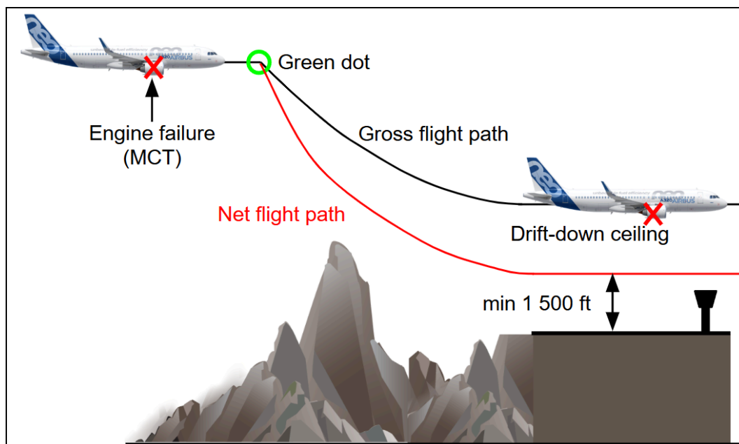
Illustration E-6: Performance Requirement above Diversion Airport
