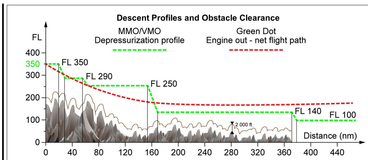
Illustration E-13: A319 Descent Profiles - Engine + Cabin Pressurization Failures - Air OPS CAT.IDE.A.230 allowance included
