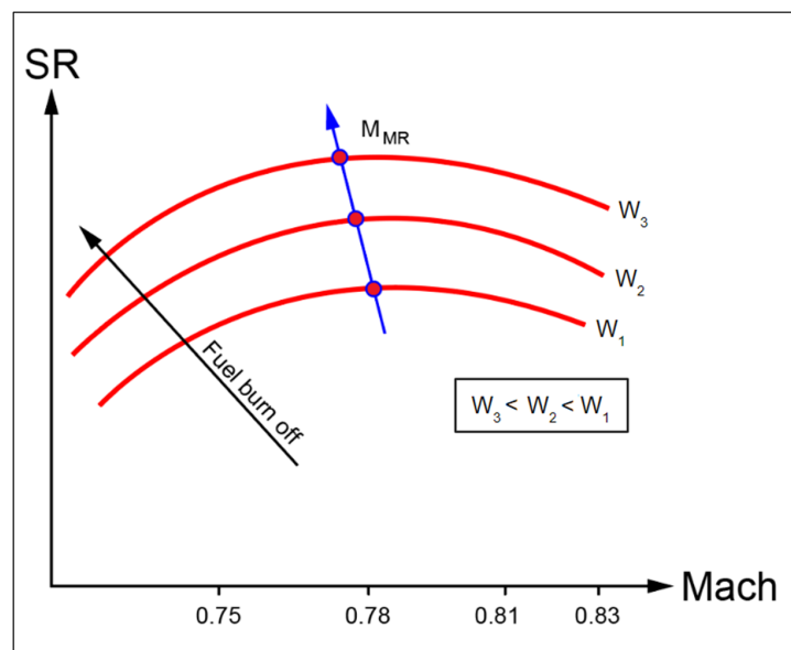
Illustration D-6: M_{MR} vs. Weight at Fixed Altitude
