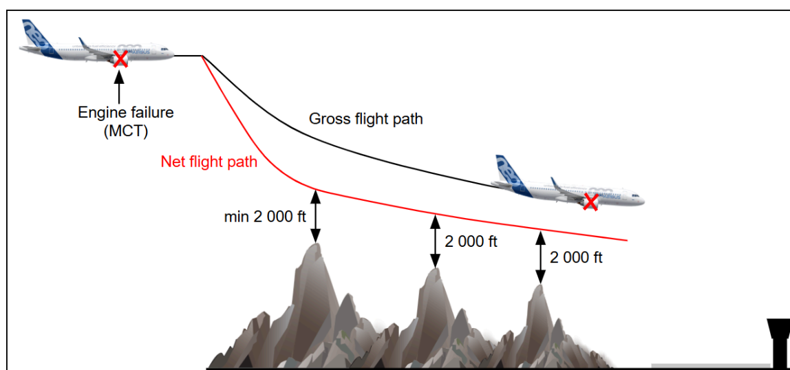
Illustration E-5: Vertical Clearance (2 000 feet)
