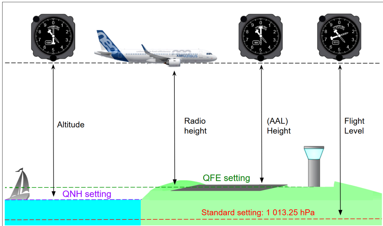
Illustration A3-4: QNH and Pressure Altitude
