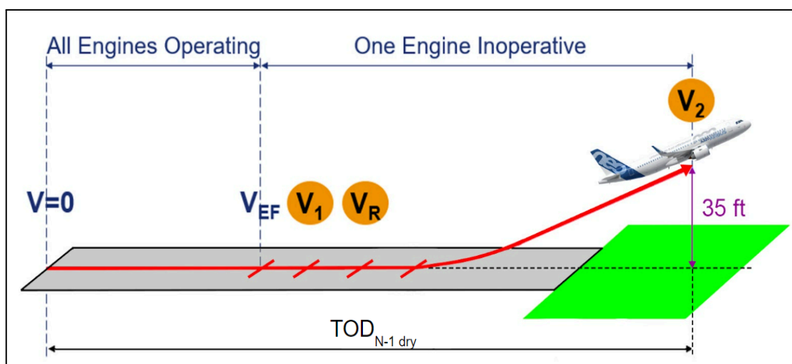
Illustration C-12: TOD_{N-1 \text{ dry}}
